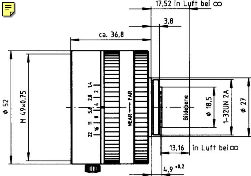
Xenoplan 1,4/17 in man. Blendenkörper
